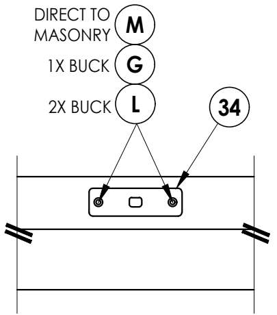
DETAIL 1 Astragal Shootbolt Strike Plate @ Head
