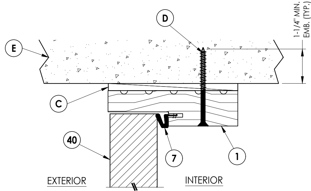
2 VERTICAL CROSS SECTION 6 Shown Direct to Masonry Outswing only
