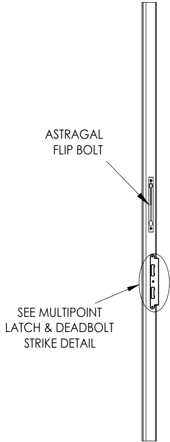
ASTRAGAL STRIKE Multipoint Lock
