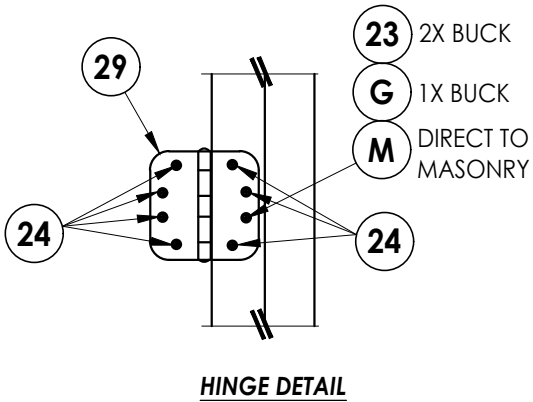
HINGE DETAIL
