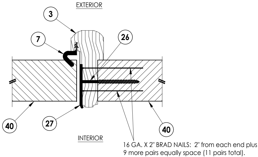
3 HORIZONTAL CROSS SECTION Inswing shown (Outswing similar)
