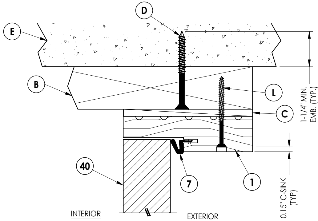
2 VERTICAL CROSS SECTION Shown w/ 2X Buck Inswing shown (Outswing similar)
