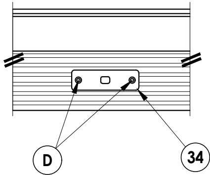
DETAIL 2 Astragal Shootbolt Strike Plate @ Sill (Outswing)
