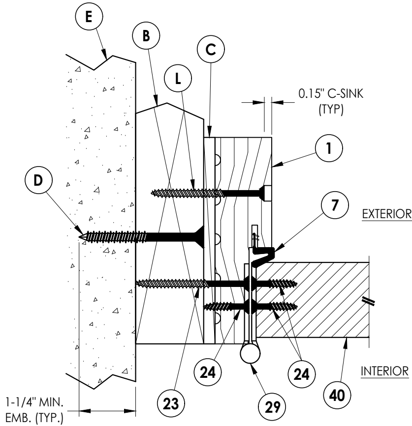
1 HORIZONTAL CROSS SECTION Shown w/ 2X Buck Inswing shown (Outswing similar)
